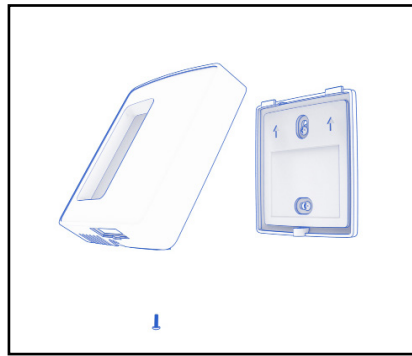
Once back plate is mounted, attach the face plate and affix security screw to the bottom.
