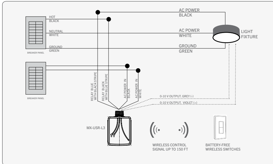
FIGURE B: Dual Power Source
